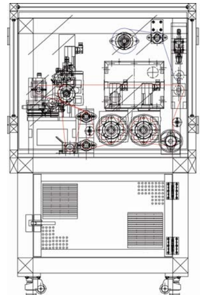
Drawing Coatema Smartcoater
