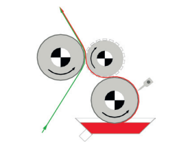
Flexography system
