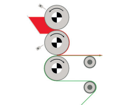
Reverse Roll system
