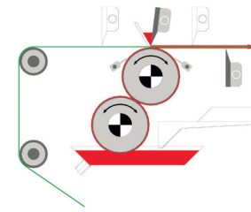
Double Side system
