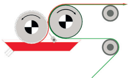
Engraved roller system
