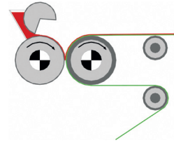
Reverse commabar system
