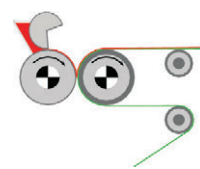
Reverse commabar system
