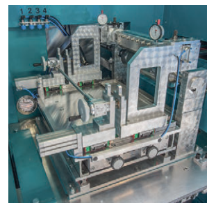
Slot die module on trolley system
