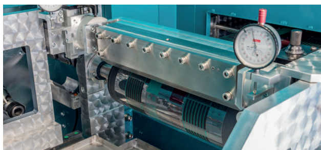
Slot die module on trolley system
