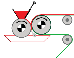
Case knife system
