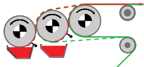
3-roller combi coating system
