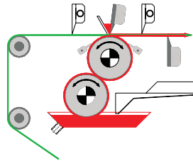
Double side coating system
