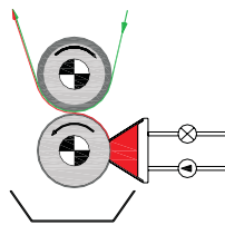
Gravure roller system
