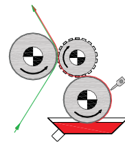
Flexography system
