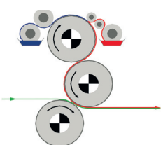
Offset lithography system
