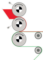
Reverse roll coating system
