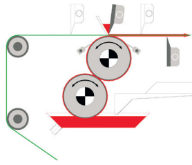
Double side coating system
