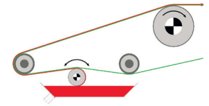
Micro roller coating system
