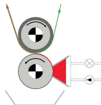
Gravure roller system
