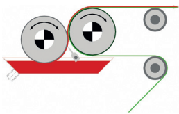
2-roller coating system
