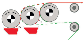
3-roller combi coating system
