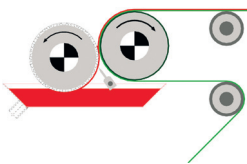
Engraved roller system
