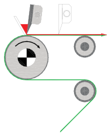
Doctor blade system
