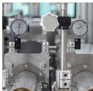
Engraved roller system
